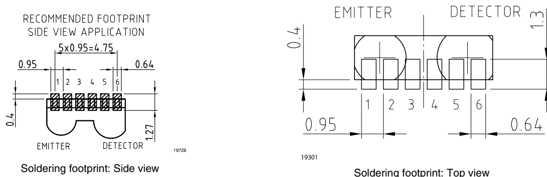
Figure 8. Soldering footprints
