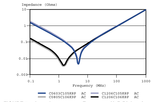
FIGURE 7. Impedance versus Frequency X5R Dielectric
