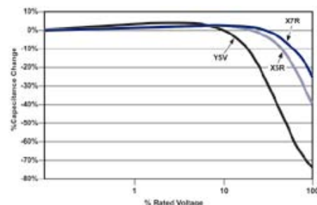
Figure 8 - Typical Variation of Capacitance with Applied DC Voltage (tension factor change.)
