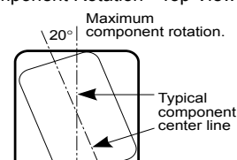
Sketch C: Component Rotation - Top View
