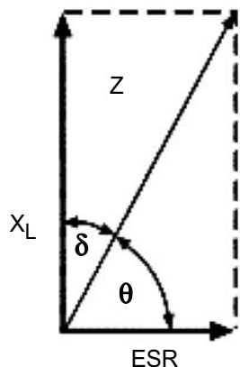
Figure 2b Total Impedance of the Capacitor Above Resonance
