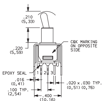
T101MH9V3BE SPDT
