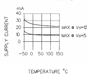
SUPPLY CURRENT VERSUS TEMP
