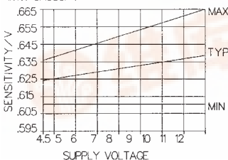
SENSITIVITY/V VERSUS SUPPLY VOLTAGE (mV/GAUSS/V)
