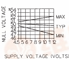
RATIO OF Vnull TO Vsupply
