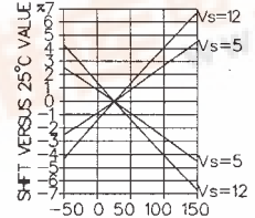
TYPICAL NULL SHIFT VERSUS TEMP
