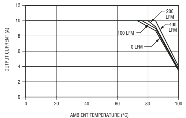
Temperature Derating
