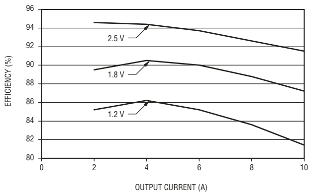
Efficiency Curve
