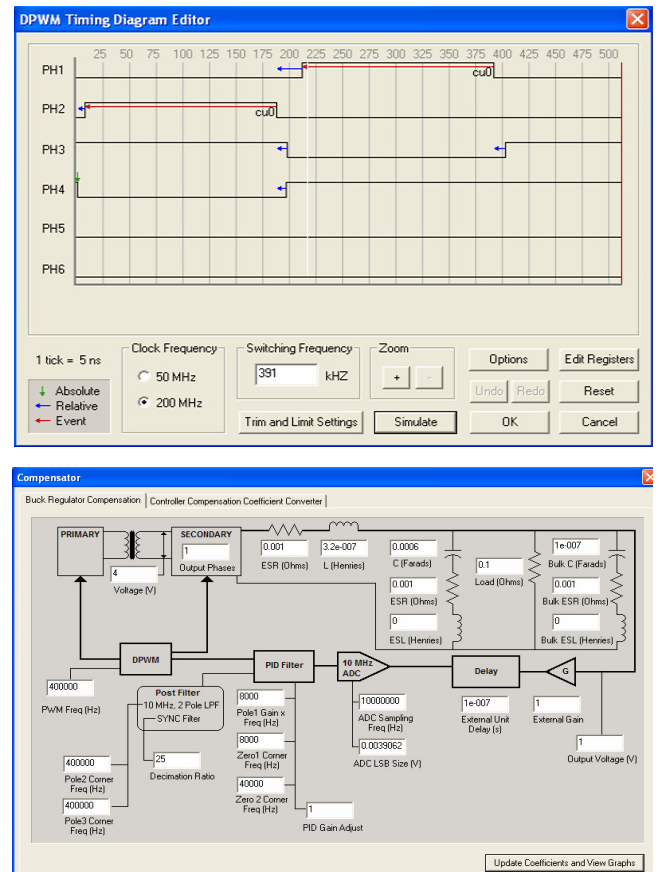
Figure 5. Timing Design Tool (Top) and Buck Regulator Compensation Tool (Bottom)
