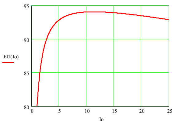
Figure 8. POL Efficiency
