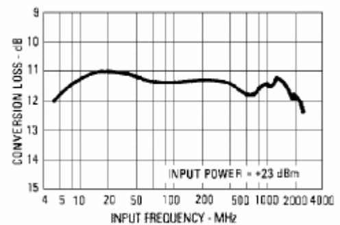
Conversion Loss vs. Input Frequency
