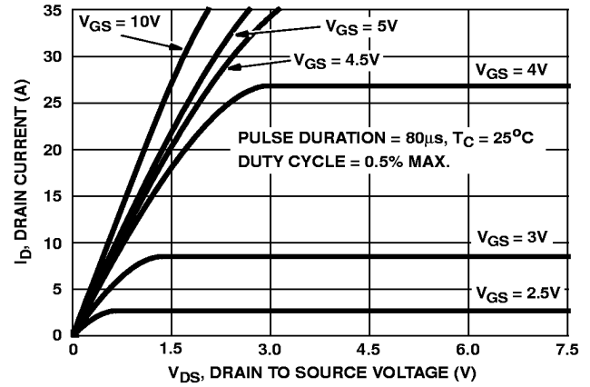
FIGURE 7. SATURATION CHARACTERISTICS
