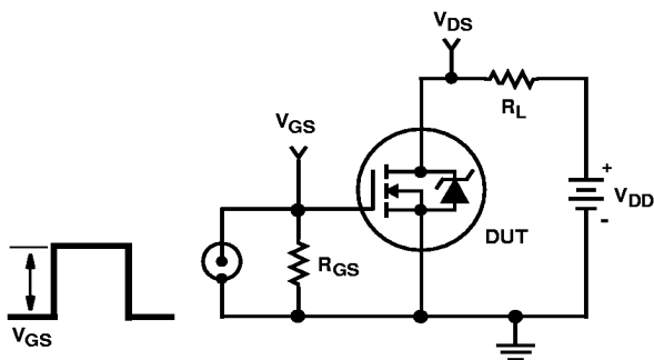
FIGURE 18. SWITCHING TIME TEST CIRCUIT
