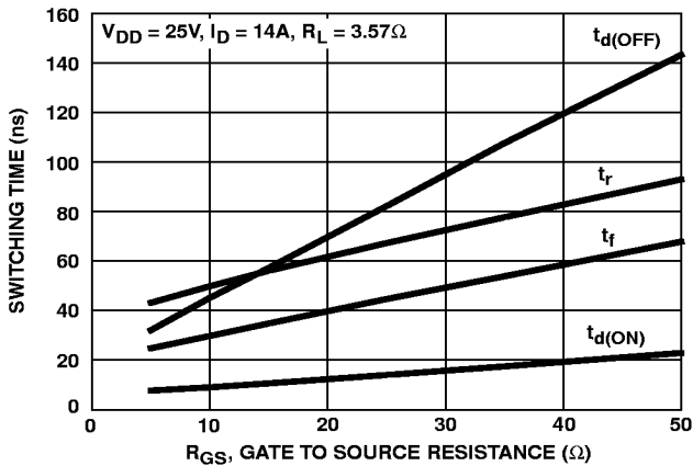
FIGURE 10. SWITCHING TIME vs GATE RESISTANCE
