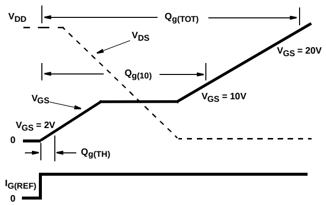
FIGURE 20. GATE CHARGE WAVEFORM
