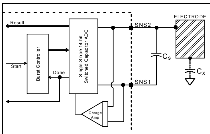
Figure 1-2 Internal Switching & Timing
