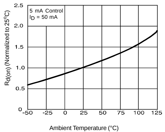
Figure 2. Typical On-Resistance
