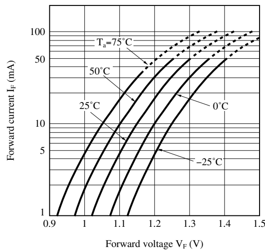
Fig.3-b Forward Current vs. Forward Voltage (Rank 2)
