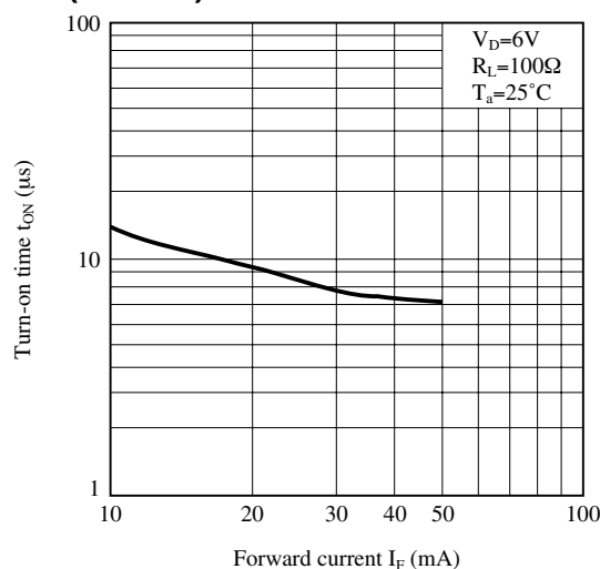
Fig.9-a Turn-on Time vs. Forward Current (Rank 1)
