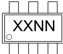
6-Lead SOT-23A*
