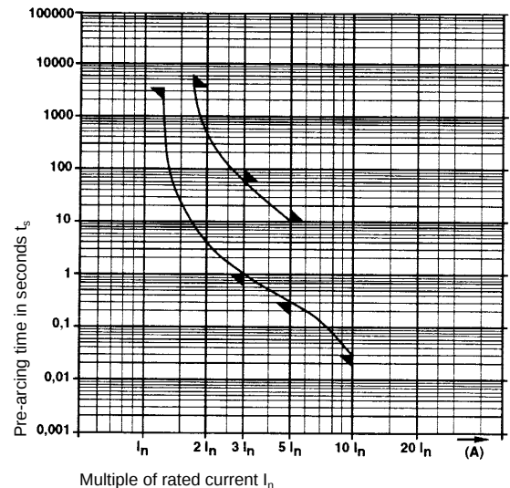
Thermal characteristics without current
