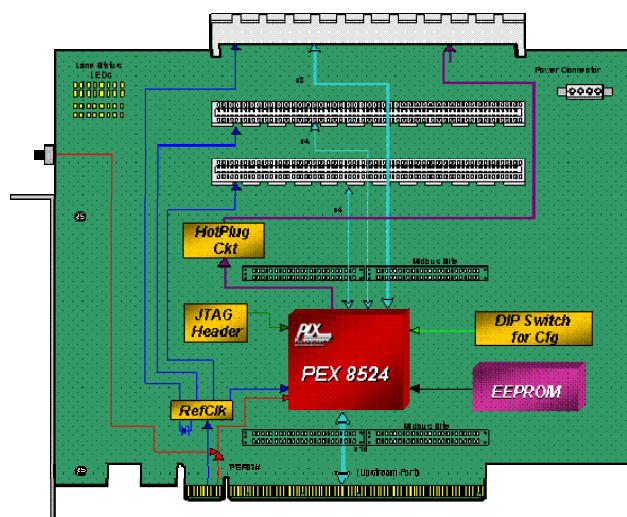
Figure 8. PEX 8524RDK
