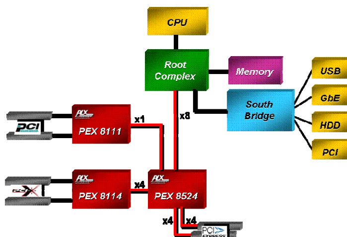
Figure 2. Fan-in/out Usage
