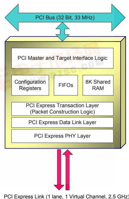
Figure 1. PEX 8111 Block Diagram
