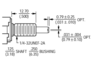
F Style Bushing
