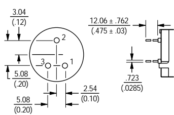
PC PIN TERMINAL
