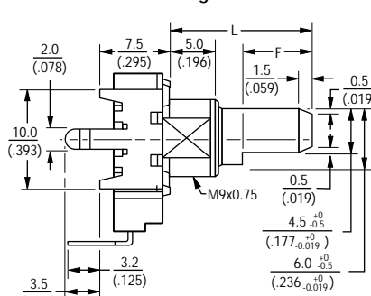
PTV142B-4 With Bushing
