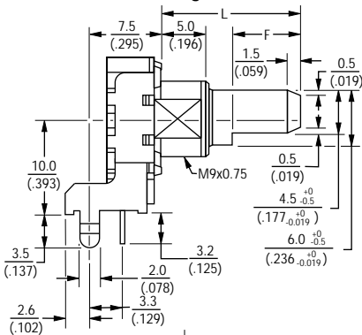
PTV142B-2 With Bushing
