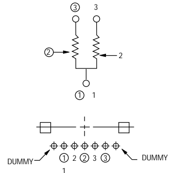
"Y" WITH TAP
