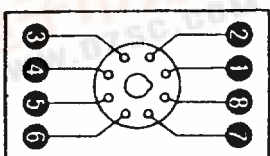
Terminal Arrangement (Top View)
