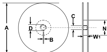
Reel Dimension
