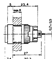
Terminals
