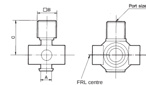
DIMENSIONS T TAKE OFF
