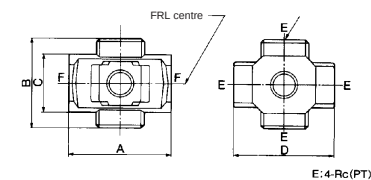
DIMENSIONS X TAKE OFF
