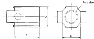
DIMENSIONS PIPING ADAPTOR
