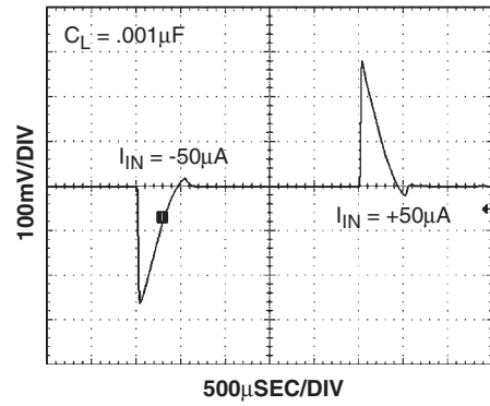
50μA LOAD TRANSIENT RESPONSE
