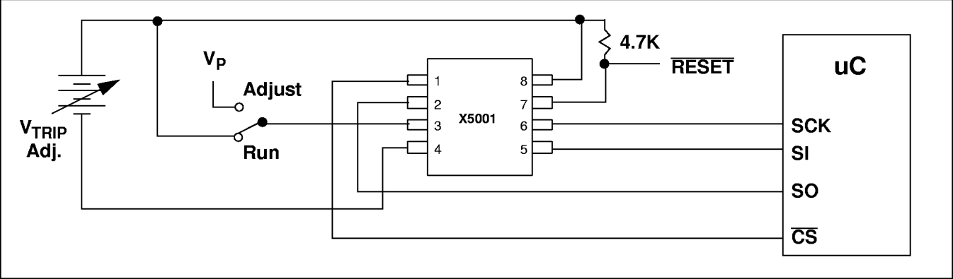
Figure 3. Set V_{TRIP} Level Sequence ( V_{CC} =desired V_{TRIP} value.)
