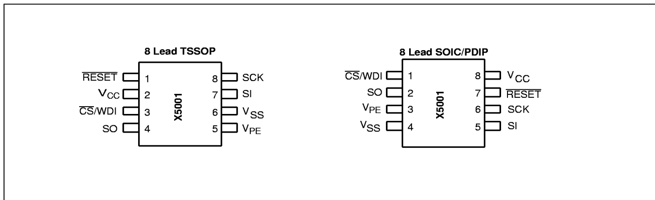
Figure 1. PIN CONFIGURATION
