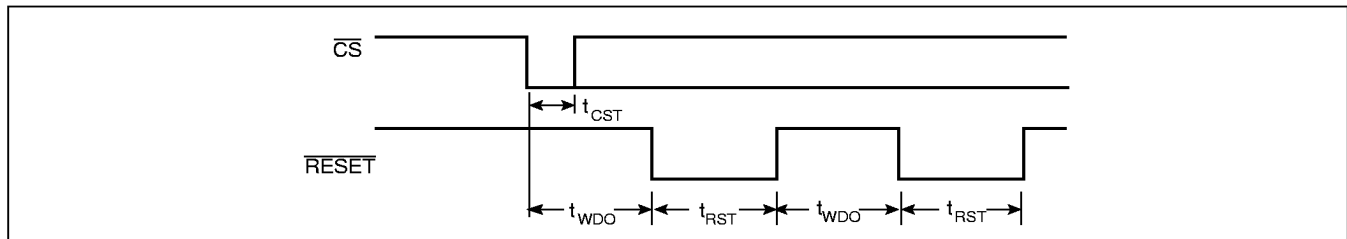
Figure 2. \overline{CS} vs. RESET Timing
