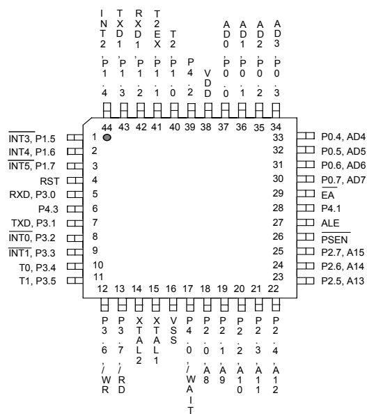
44-Pin QFP
