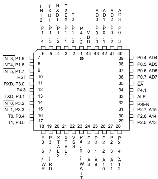
44-Pin PLCC
