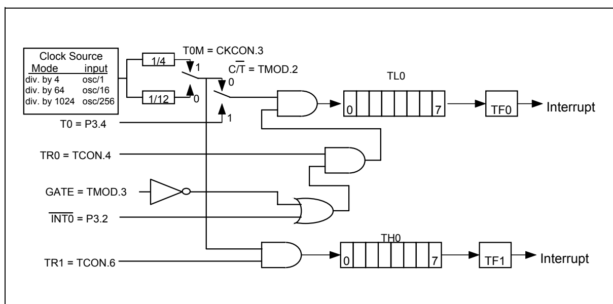
Figure 13. Timer/Counter 0 Mode 3
