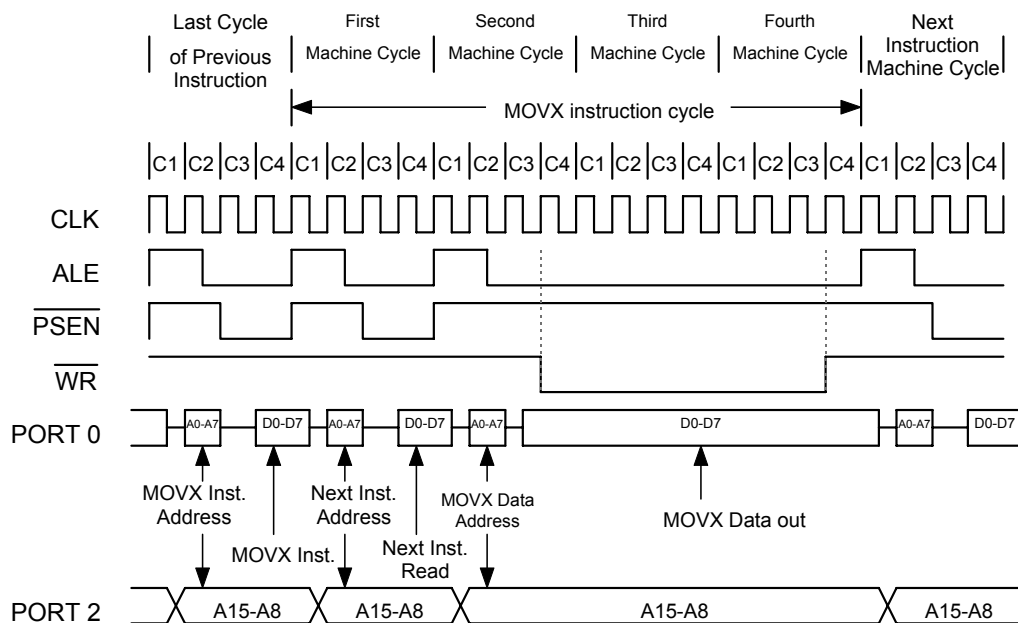
Figure 10. Data Memory Write with Stretch Value = 2
