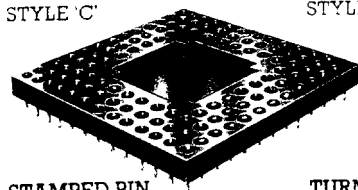
STAMPED PIN SOLDER TAIL
