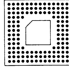
WP(X)136A1414(XXX) STYLES AVAILABLE A/B/C/D
