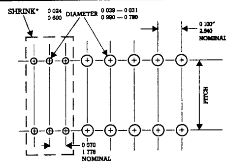
RECOMMENDED MOUNTING HOLE PATTERNS
