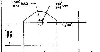
W5811 PLASTIC TO3
