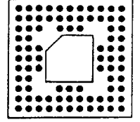
WP(X)85A1111(XXX) STYLES AVAILABLE A/B/C/D/E/F
