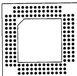
WP(X)146A1717(XXX) STYLES AVAILABLE A/B/C/D
