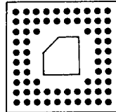
WP(X)68A1010(XXX) STYLES AVAILABLE A/B/C/D
