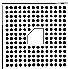
WP(X)181A1414(XXX) STYLES AVAILABLE A/B/C/D
