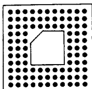
WP(X)96A1111(XXX) STYLES AVAILABLE A/B/C/D/E/F
