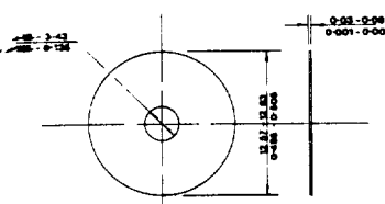
452.2 CASE 77
