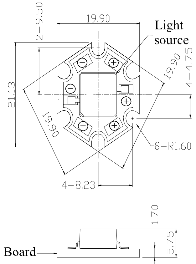
CMDA31xx15D13L Star Configuration
