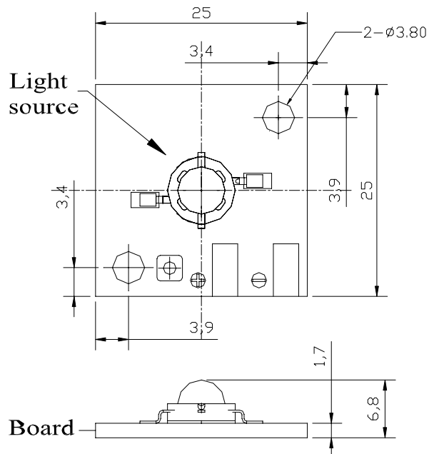
CMDA44xx15D13L Square Configuration
