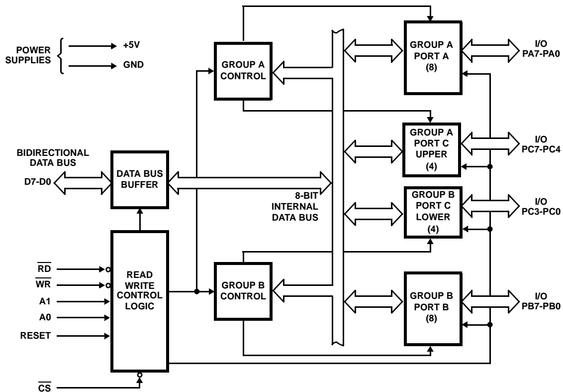
FIGURE 1. FUNCTIONAL DIAGRAM
