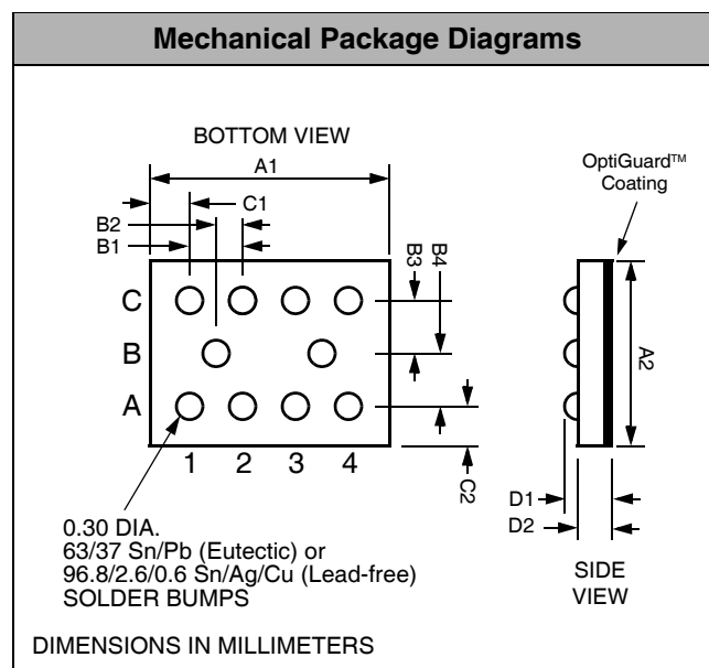
Package Dimensions for CM1426-04 Chip Scale Package
