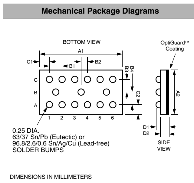
Package Dimensions for CM1441 Chip Scale Package
