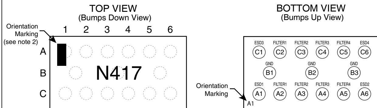
CM1441-07CS/CP 15 Bump CSP Package
