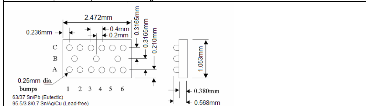
CM1452-06 (6-channel) mechanical diagram.
