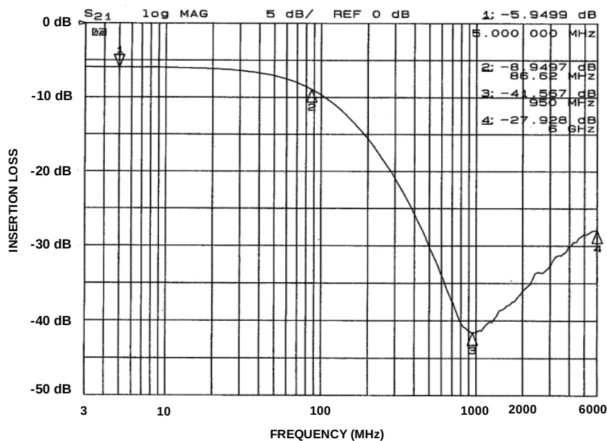
Figure 6. Insertion Loss vs. Frequency (FILTER6 Input to GND, CM1621-06DE) Typical Diode Capacitance vs. Input Voltage
