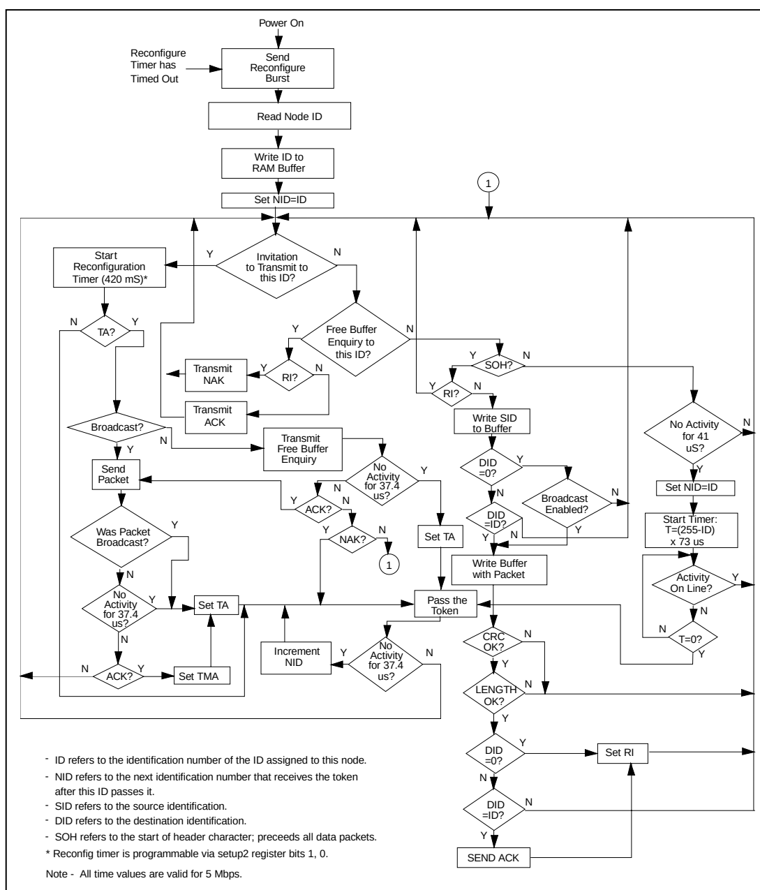
Figure 3.1 - COM20020ID Operation
