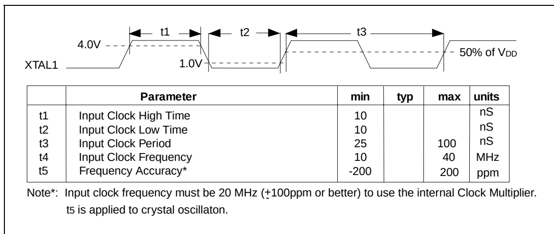
Figure 8.13 - TTL Input Timing on XTAL1 Pin
