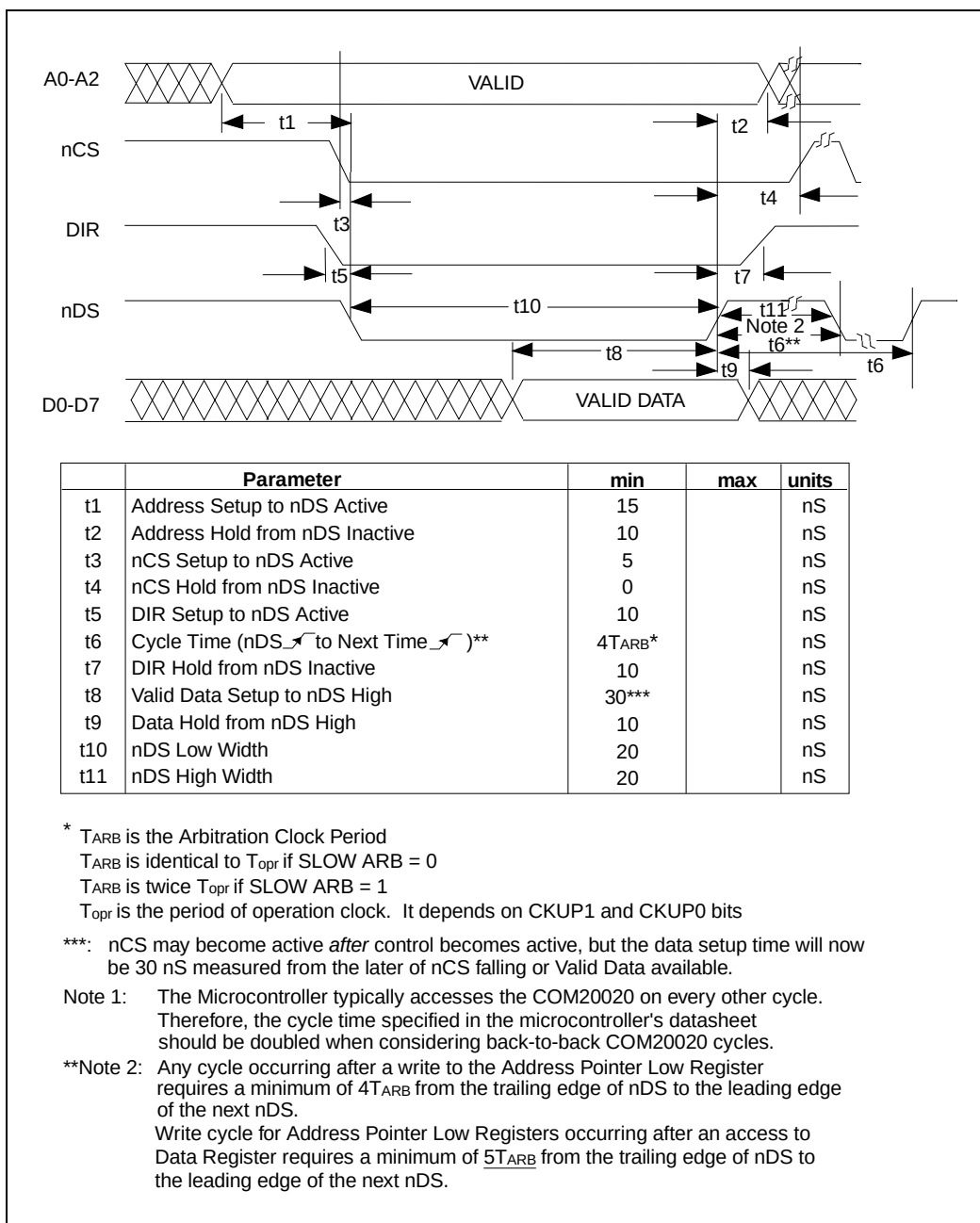
Figure 8.10 - Non-Multiplexed Bus, 68XX-Like Control Signals; Write Cycle
