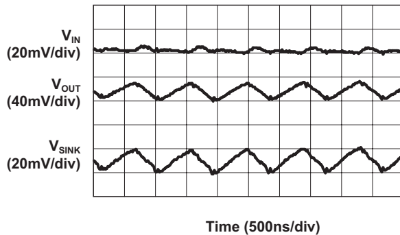
Backlight Operating Characteristic ( V_{IN} = 3.5V ; 1.5X Mode; 13.5mA/ch Load)
