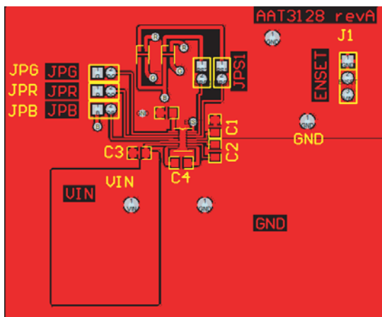
Figure 3: AAT3128 Evaluation Board Component Side PCB Layout.
