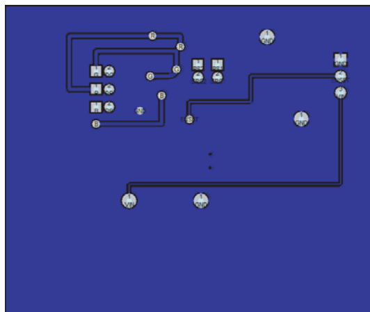
Figure 4: AAT3128 Evaluation Board Solder Side PCB Layout.
