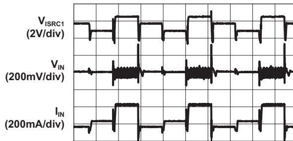
Input vs. Output Transient ( V_{IN} = 4.2V ; Data 5)
