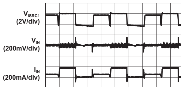
Input vs. Output Transient ( V_{IN} = 2.7V ; Data 5)
