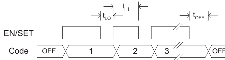
Figure 1: S 2 Cwire Timing Diagram.
