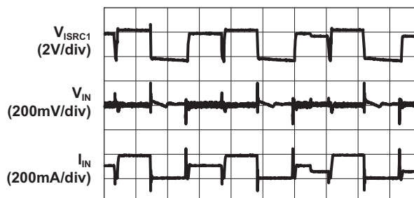
Input vs. Output Transient ( V_{IN} = 3.6V ; Data 5)
