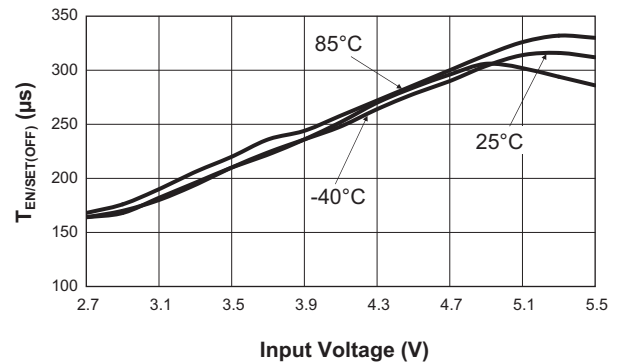
EN/SET Input OFF Timeout vs. Input Voltage
