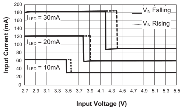
Input Current vs. Input Voltage (Excluding AAT3193-4, PWM Option)
