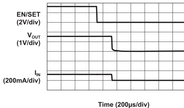
Turn Off from 2X Mode (20mA/ch)
