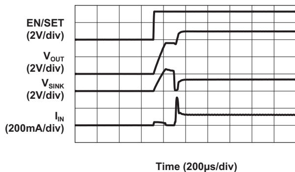
Turn On to 2X Mode (20mA/ch)
