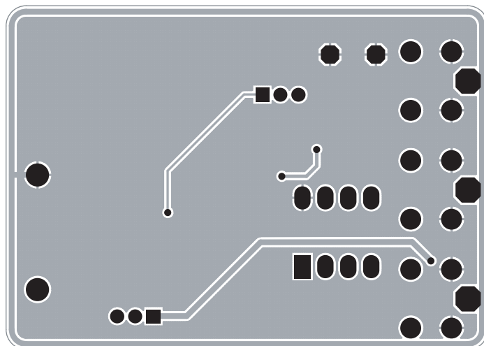
Figure 9: AAT3193 Evaluation Board Solder Side Layout.
