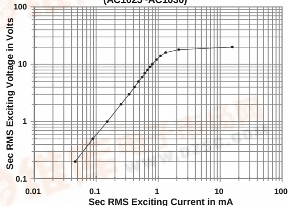
Typical Excitation Curve (AC1025-AC1030)
