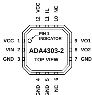
Figure 4. Pin Configuration
