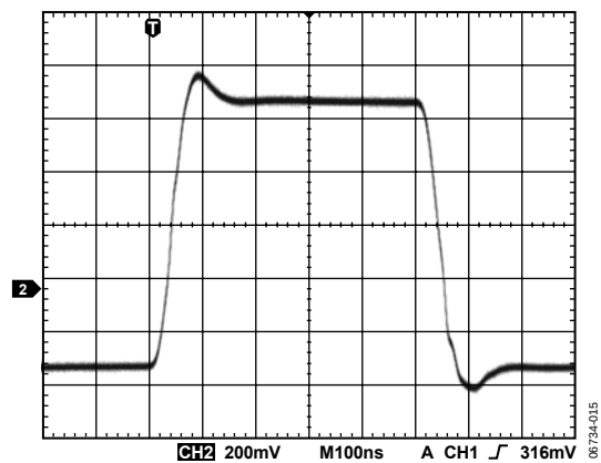
Figure 14. Transient Response
