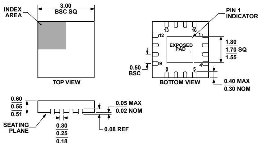
Figure 20. 16-Lead Lead Frame Chip Scale Package [LFCSP_UQ] 3 mm × 3 mm Body, Ultra Thin Quad (CP-16-12)
