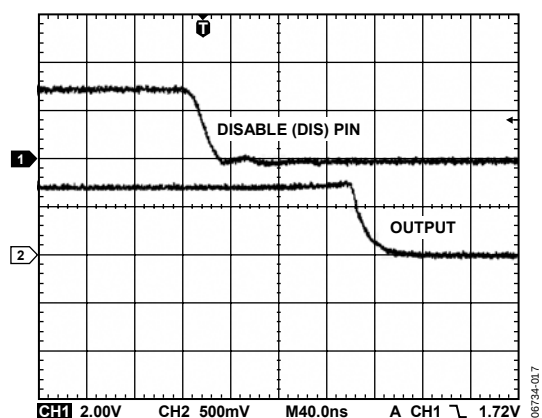
Figure 16. Output Disable
