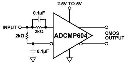
Figure 21. Self-Biased, 50% Slicer
