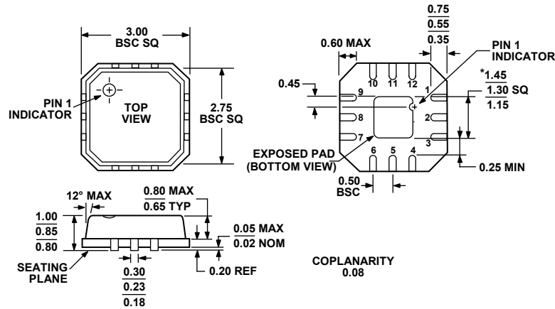
Figure 28. 12-Lead Lead Frame Chip Scale Package (LFCSP_VQ)
