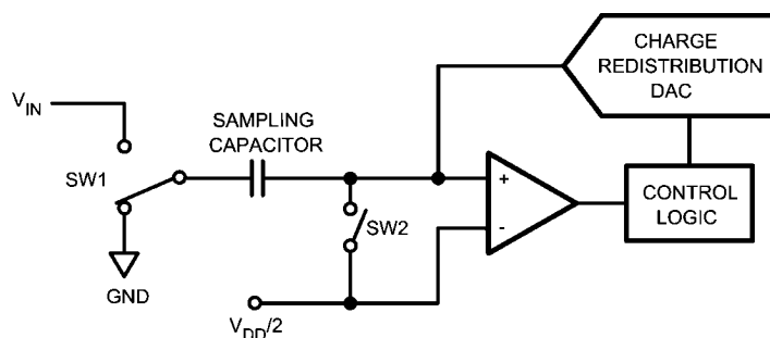
FIGURE 5. ADCS7476/77/78 in Hold Mode
