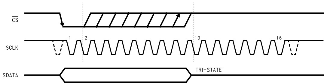
FIGURE 10. Entering Shutdown Mode
