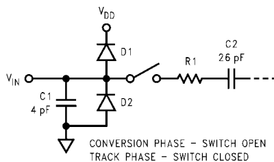
FIGURE 9. Equivalent Input Circuit
