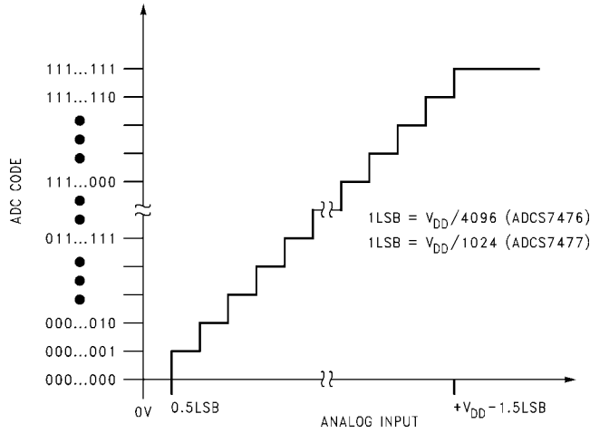
FIGURE 6. ADCS7476/77 Ideal Transfer Characteristic
