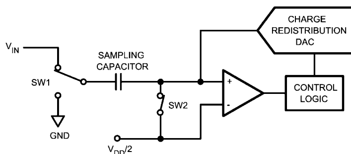
FIGURE 4. ADCS7476/77/78 in Track Mode
