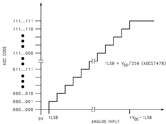
FIGURE 7. ADCS7478 Ideal Transfer Characteristic
