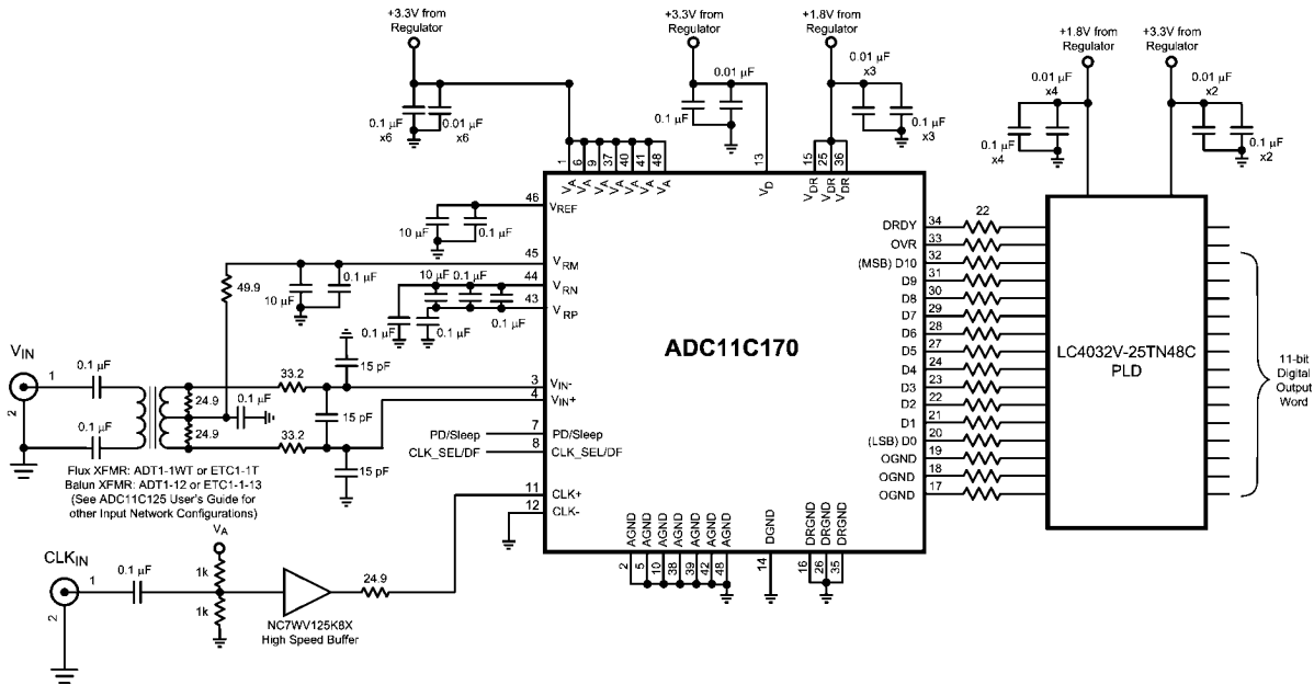
FIGURE 4. Application Circuit using Transformer Drive Circuit. If 14-bit compatibility is not required do not connect pins 17 - 19. If 12-bit compatibility if not required do not connect pin 19.
