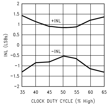
INL vs. Clock Duty Cycle
