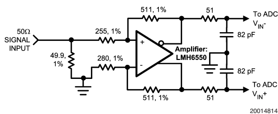
FIGURE 5. Differential Drive Circuit of Figure 4
