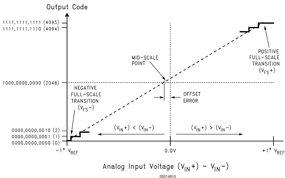
FIGURE 1. Transfer Characteristic
