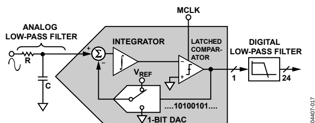
Figure 19. First-Order, \Sigma - \Delta ADC
