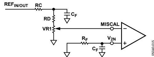
Figure 17. Typical Connection for MISCAL
