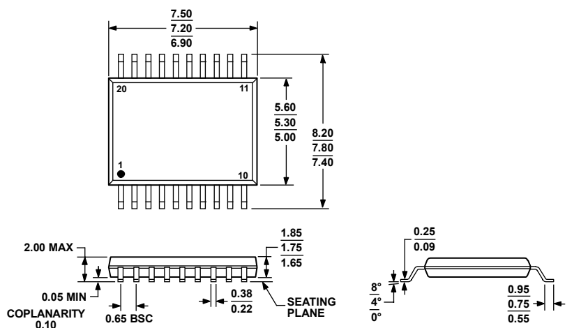
Figure 36. 20-Lead Shrink Small Outline Package [SSOP] (RS-20)
