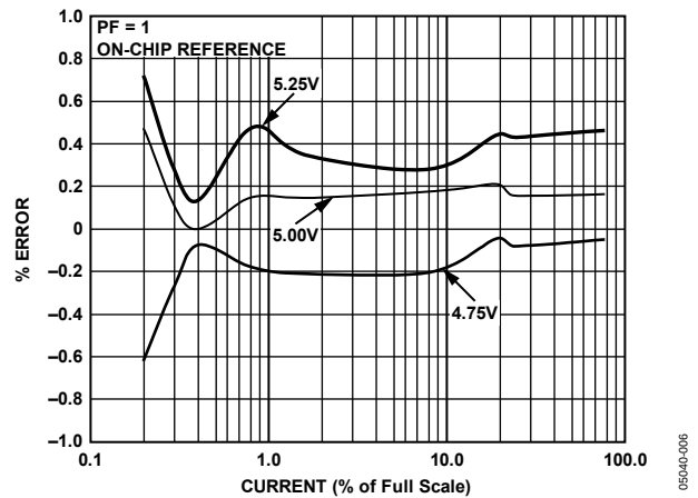
Figure 8. Active Power Error as a Percentage of Reading over Power Supply with Gain = 1 and Internal Reference
