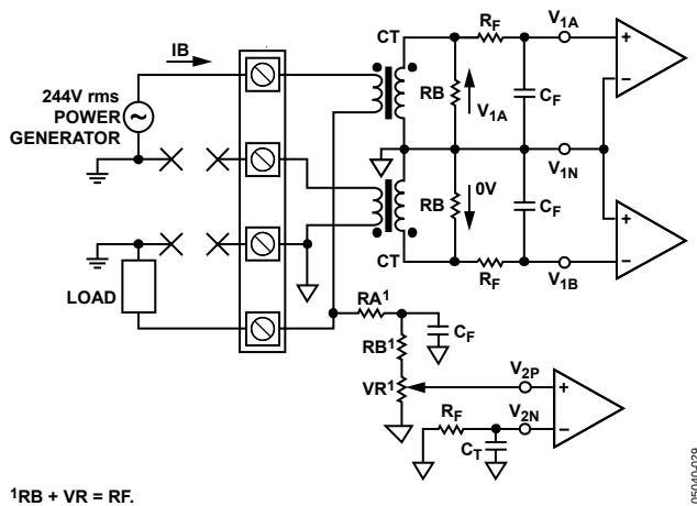
Figure 31. Missing Neutral System Diagram
