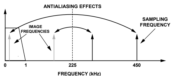
Figure 21. ADC and Signal Processing in Current Channel or Voltage Channel
