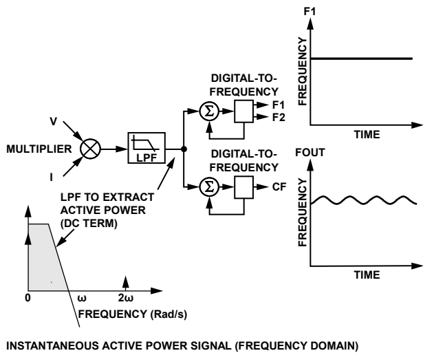
Figure 27. Active Power to Frequency Conversion
