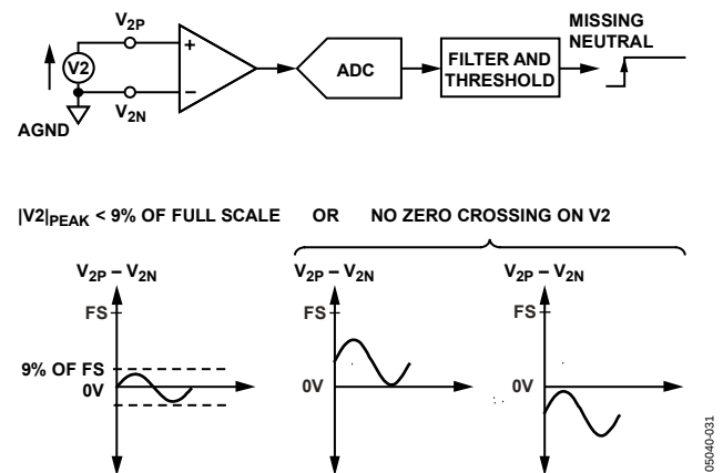
Figure 33. Missing Neutral Detection
