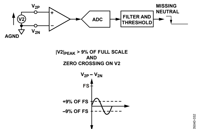
Figure 34. Return to Normal Mode after Missing Neutral Detection
