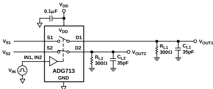
Test Circuit 5. Break-Before-Make Time Delay
