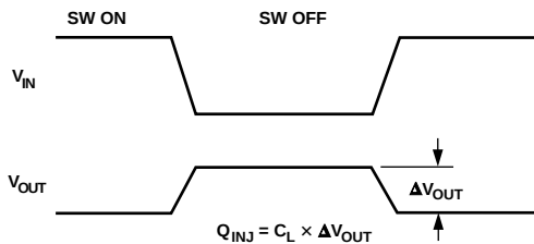
Test Circuit 6. Charge Injection
