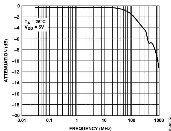
Figure 15. Bandwidth
