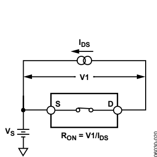
Figure 22. On Resistance
