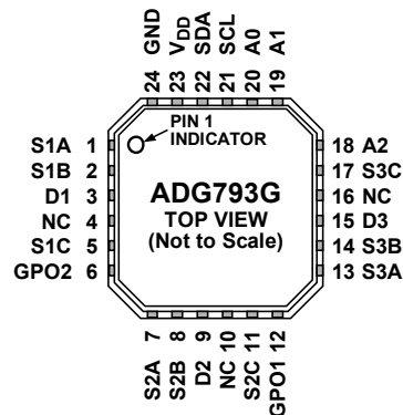
Figure 4. ADG793G Pin Configuration
