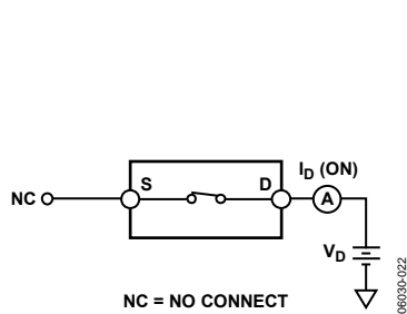
Figure 23. Off Leakage
