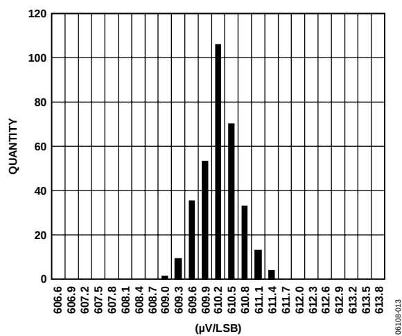
Figure 13. DAC Gain Distribution at 25°C/3.3 V
