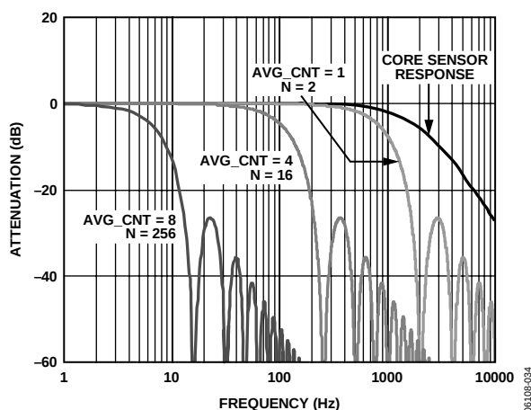
Figure 30. INCL_OUT, INCL_180_OUT Filter Response
