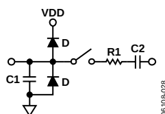
Figure 32. Equivalent Analog Input Circuit Conversion Phase: Switch Open Track Phase: Switch Closed
