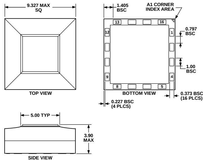
Figure 36. 16-Terminal Land Grid Array [LGA] (CC-16-2) Dimensions shown in millimeters
