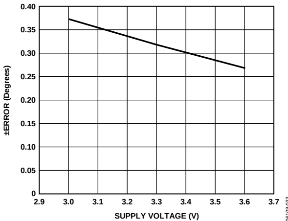
Figure 7. Inclination Error vs. Supply
