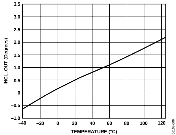
Figure 6. Inclination Error vs. Temperature
