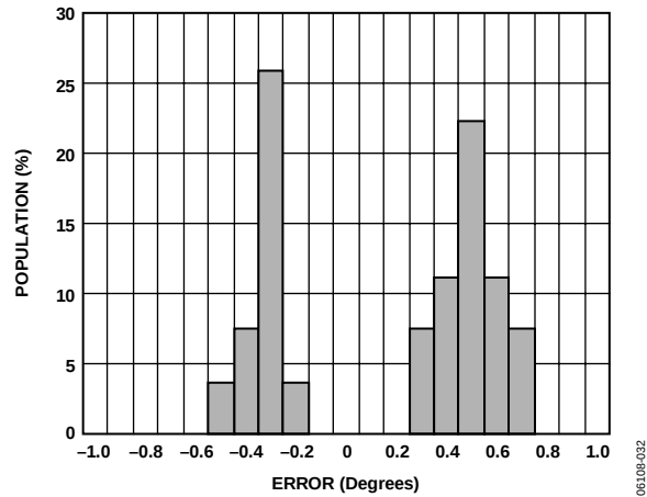
Figure 5. Inclination Error Distribution at 25°C/3.3 V, Incline = 0°
